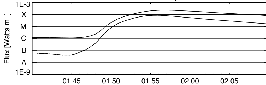
GOES 15 X-Rays:
