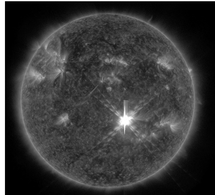
AIA131 20110215_015621
