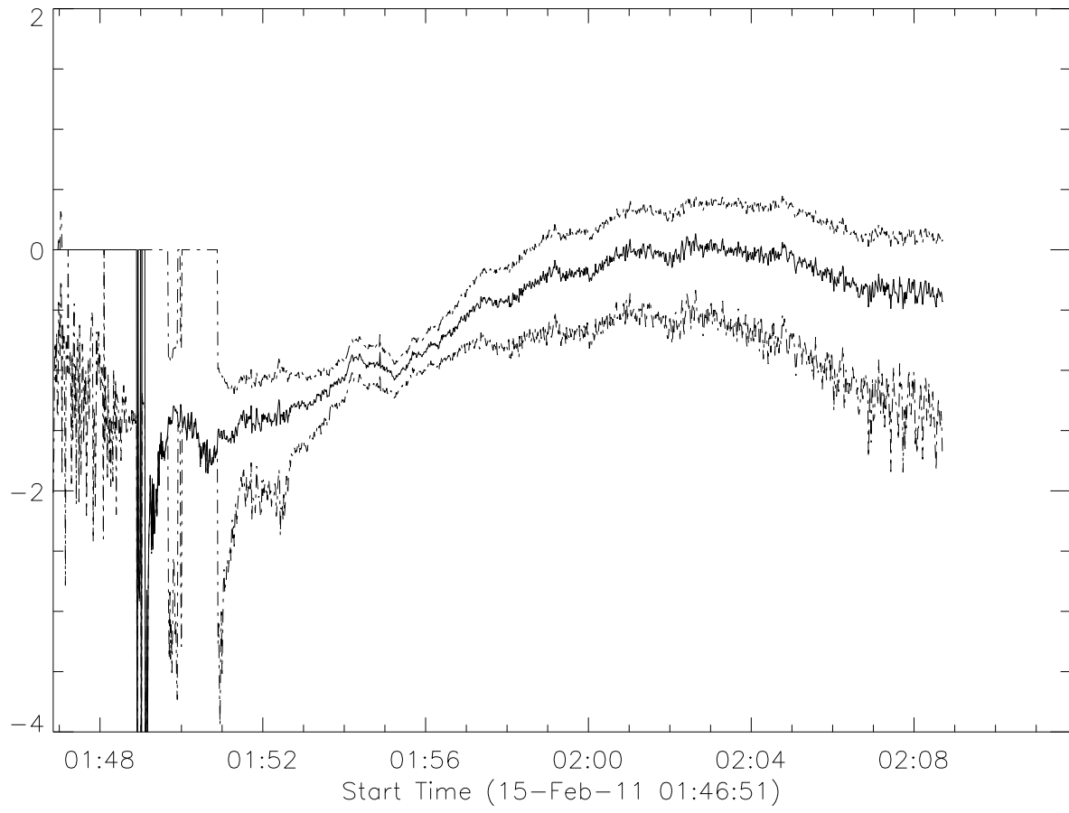
linear fit coef.1
