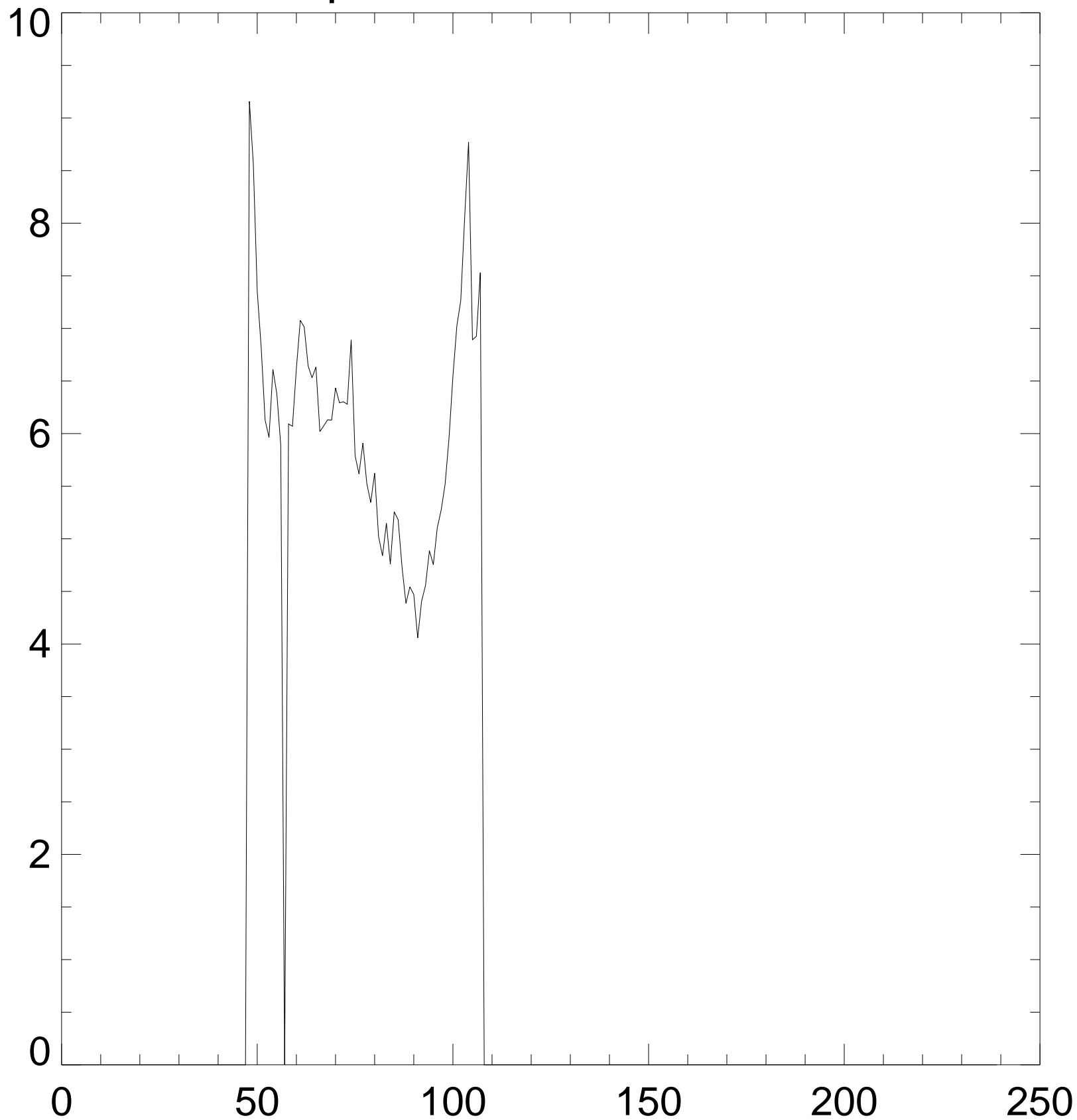
spectral index vs. time
