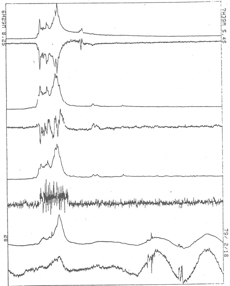
Fig. 7 Burst time profiles observed by the full-automatic radio-polarimeters on February 18, 1979. 8 channel data are from top to bottom 9.4 GHz intensity (I) and polarization (V), 3.75 GHz I and V, 2 GHz I and V, and 1 GHz I and V. Vertical peak-to-peak interval is same for each channel. Receiver gain attenuation, which is seen in Fig. 6, is recovered to obtain original profiles. Maximum time at 3.75 GHz is 0645 UT.
