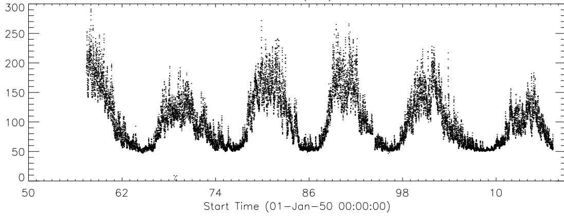
3.75GHz (sfu)
