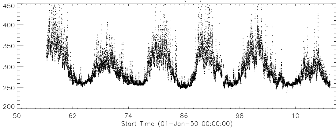
9.4GHz (sfu)
