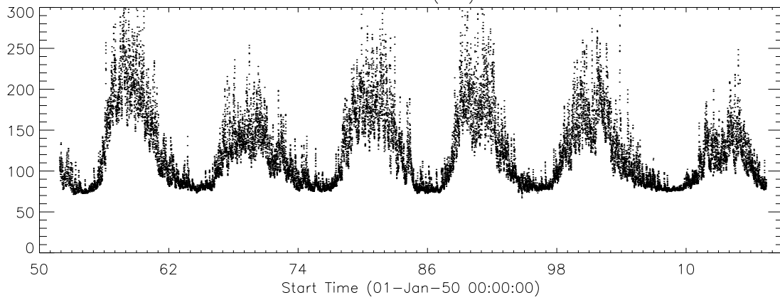
9.4GHz (sfu)
